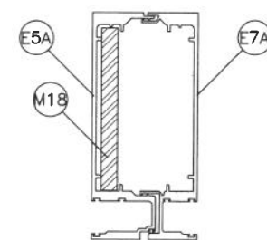
MULLION 'M3'
