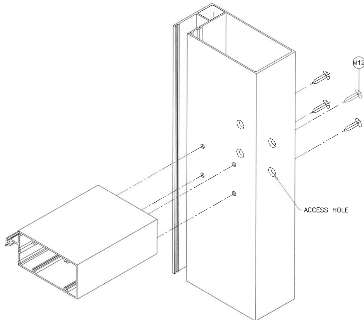
HORIZONTAL CORNER
