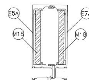
MULLION 'M4'
