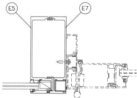
MULLION 'MD1'
